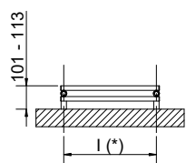
Detail of the pipe centres 50 mm version
