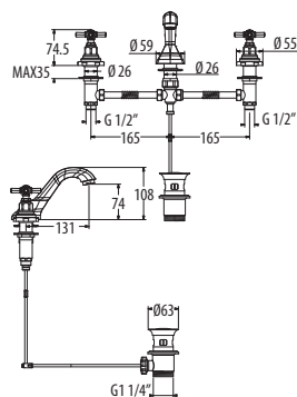
Art. 2321 vitone ceramico ceramic headwork
