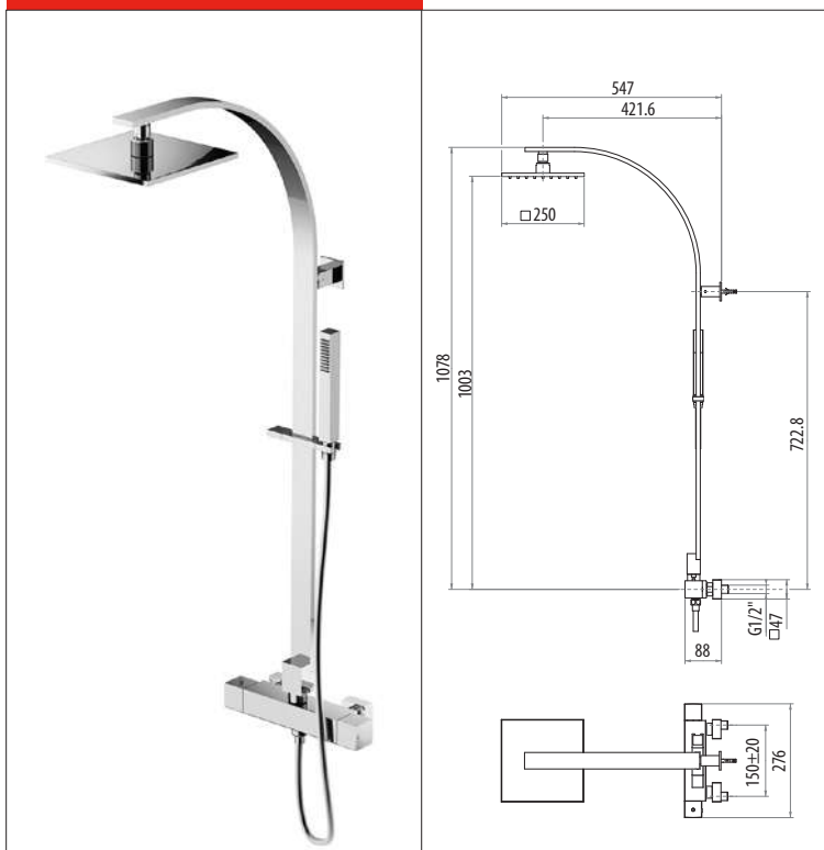
Art. 40991 termostatica thermostatic
