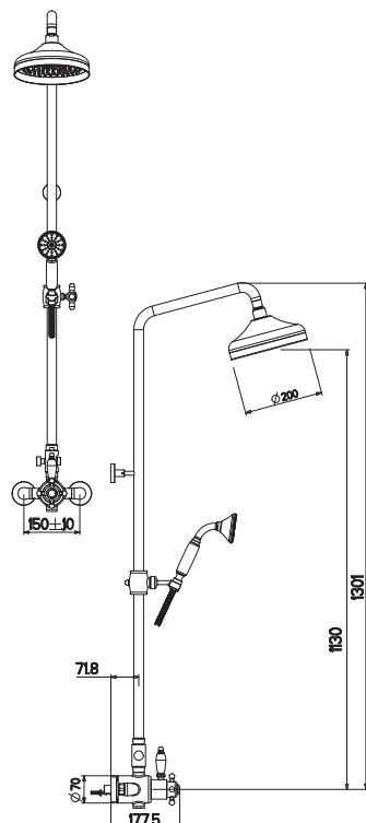
Art. 40975 termostatica thermostatic
