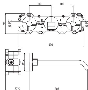
Art. 2302 vitone ceramico ceramic headwork
