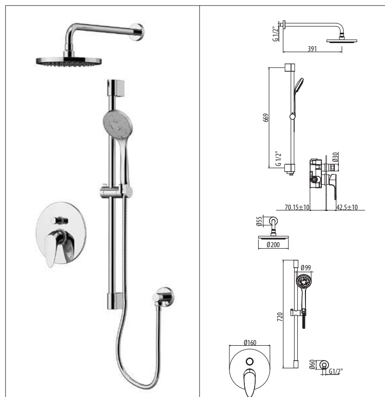
art. 6386/PD ABS 3 jets 3 getti
