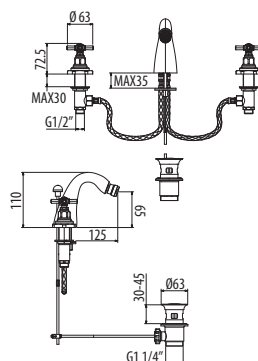
Art. 2321 vitone ceramico ceramic headwork
