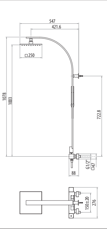
Art. 40991 termostatica thermostatic
